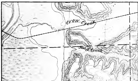
B. Map showing stream piracy east of Chillicothe. (Portion of Metamora topographic map, U. S. Geol. Surv.)
